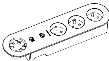
3 × 230V 2 × LAN Cat6A | cable grommet
