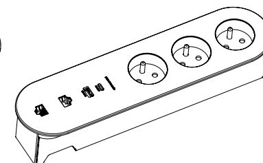
3 × 230V | USB C/A 2 × LAN Cat6A
