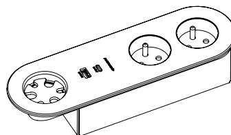
2 × 230V | USB C/A cable grommet
