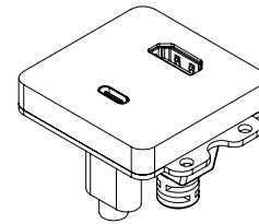
USB-C 3.2 GEN 2 M/F 10Gbps 150mm gold and nickel plated black pvc
