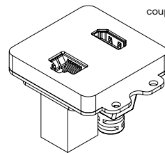
HDMI HDM12.0b F/F | 4K 60HZ 150mm | gold plated awg32/22 black pvc
