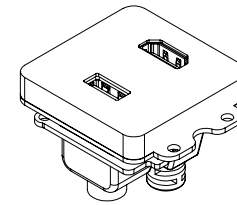
USB-A 3.0 GEN 2 F/F 5Gbps | 135mm gold and nickel plated AWG 28/28 black pvc
